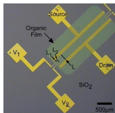
An organic thin film transistor
